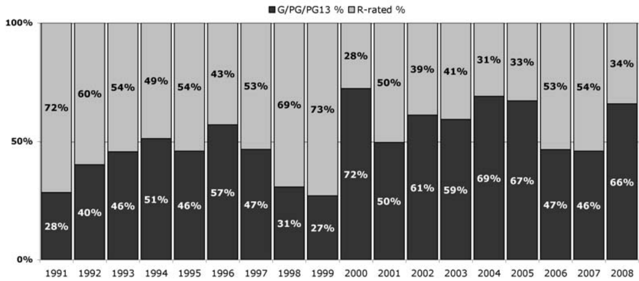
Figure 2 | Percent Youth- and R-rated Tobacco Impressions, 1991-2008
