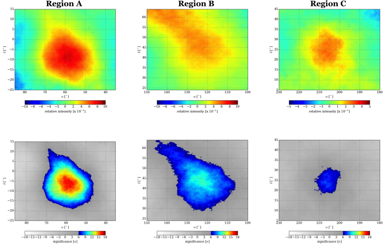
Figure 7. Relative intensity (top row) and pre-trial significance (bottom row) of the cosmic-ray flux in the vicinity of Region A (left), Region B (center), and Region C (right), from the map shown in Fig. 5.
