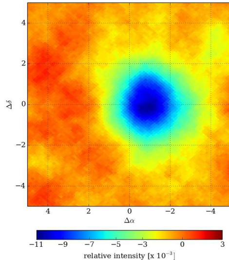
Figure 3. Relative intensity of the cosmic-ray flux in a sky map centered on the position of the Moon. \Delta\alpha and \Delta\delta are the right ascension and declination of the cosmic rays with respect to the right ascension and declination of the Moon. The Moon shadow is shown for 113 days of HAWC-95/111 data. The deficit corresponds to a significance of 24\sigma .
