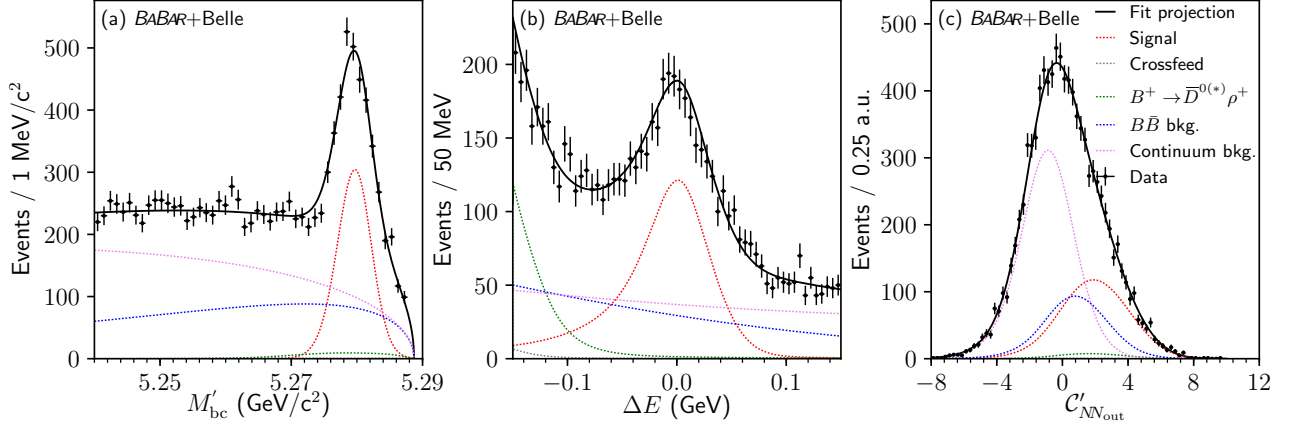
FIG. 2. (color online). Data distributions for a) M'_{bc} , b) \Delta E , and c) C'_{NNout} (points with error bars) for the BABAR and Belle data samples combined. The solid black lines represent projections of the total fit function, and the colored dotted lines show the signal and background components of the fit as indicated in the legend. In plotting the M'_{bc} , \Delta E , and C'_{NNout} distributions, each of the other two observables are required to satisfy M'_{bc} > 5.272 \text{ GeV}/c^2 , |\Delta E| < 100 \text{ MeV} , or 0 < C'_{NNout} < 8 to select signal-enhanced regions.
