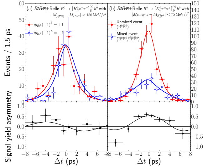
FIG. 3. (color online). Distributions of the proper-time interval (data points with error bars) and the corresponding asymmetries for B^0 \rightarrow D^{(*)} h^0 candidates associated with high-quality flavor tags for two different regions of the D \rightarrow K_S^0 \pi^+ \pi^- phase space and for the BABAR and Belle data samples combined. The background has been subtracted using the sPlot technique [49], with weights obtained from the fit presented in Fig. 2.
